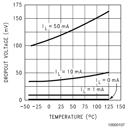
Dropout Voltage vs. Temperature
